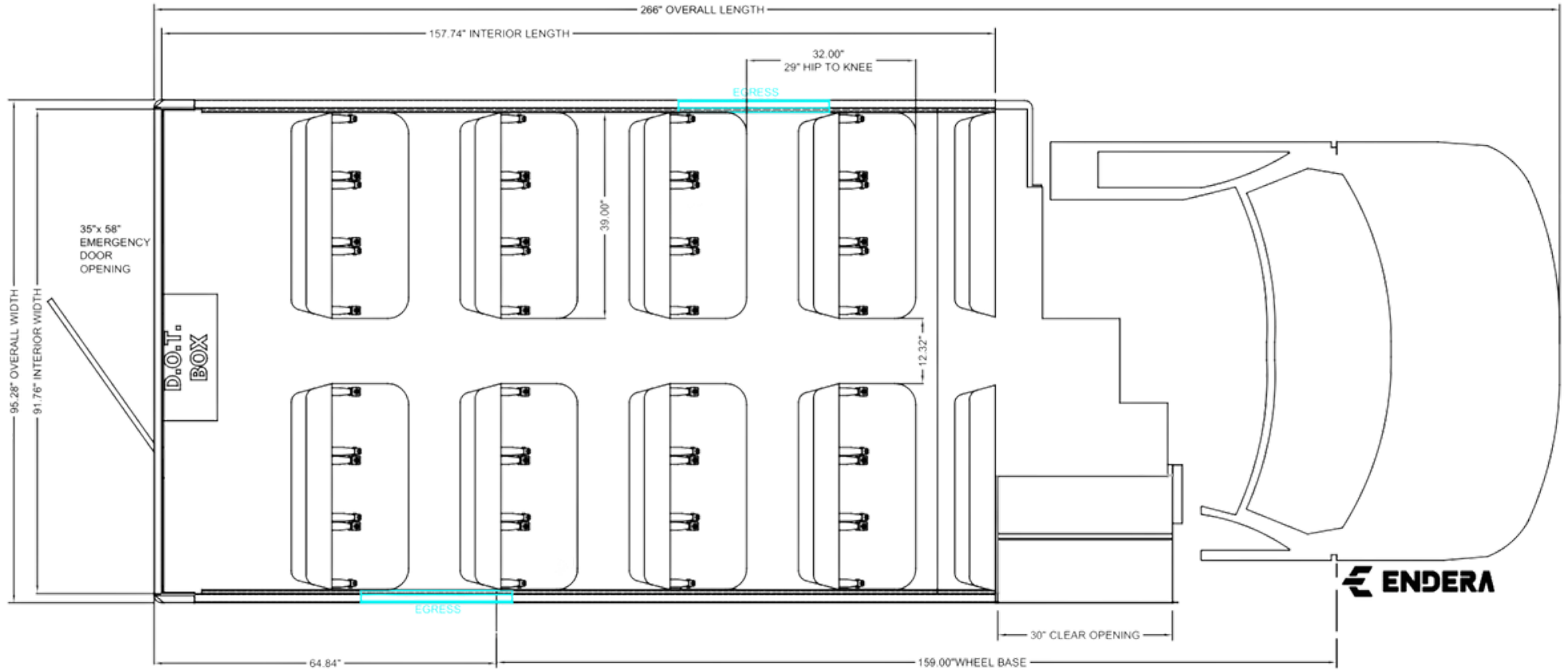
24 Passenger 5 Section Plus Driver
