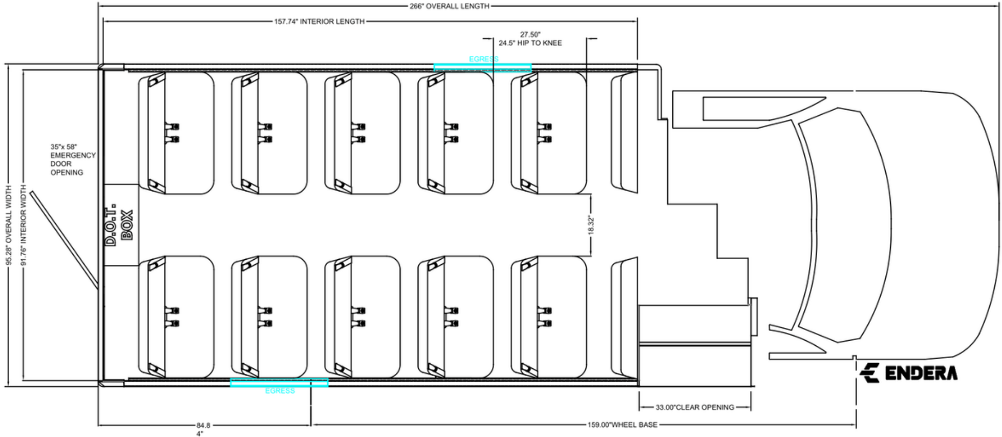
20 Passenger 5 Section Plus Driver
